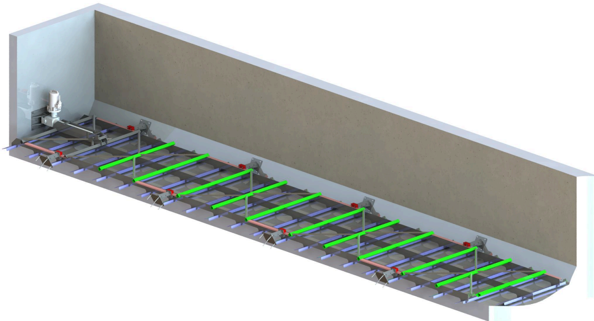
bottom scraper for gritt and sand trap EBSS made of pre-mounted segments
