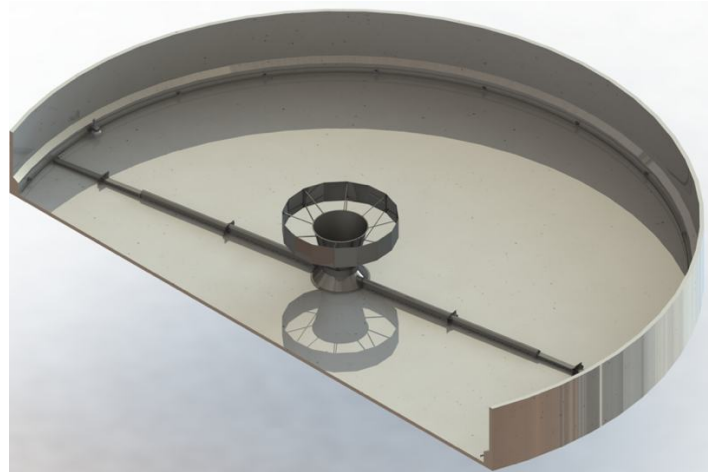
Circular suction scraper ECSS with submerged drive unit
