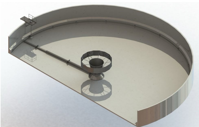
Circular suction scraper ECSS with dry placed drive unit (single arm option)
