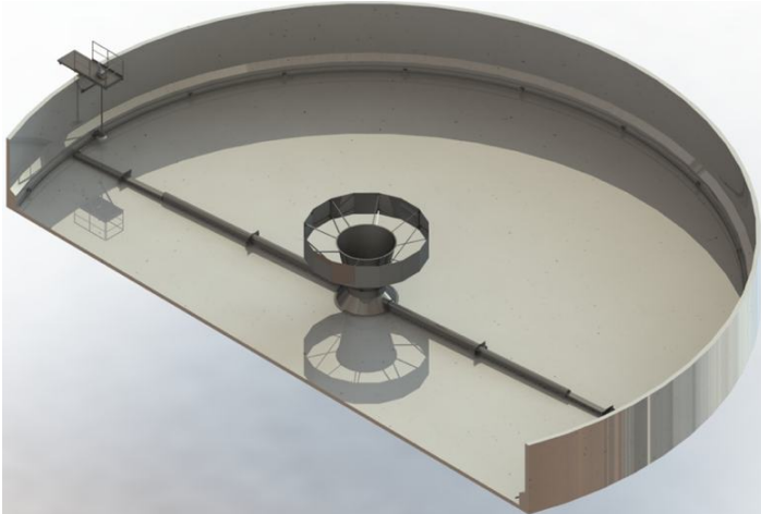
Circular suction scraper ECSS with dry placed drive unit
