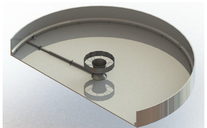
Circular suction scraper ECSS with submerged drive unit (single arm option)
